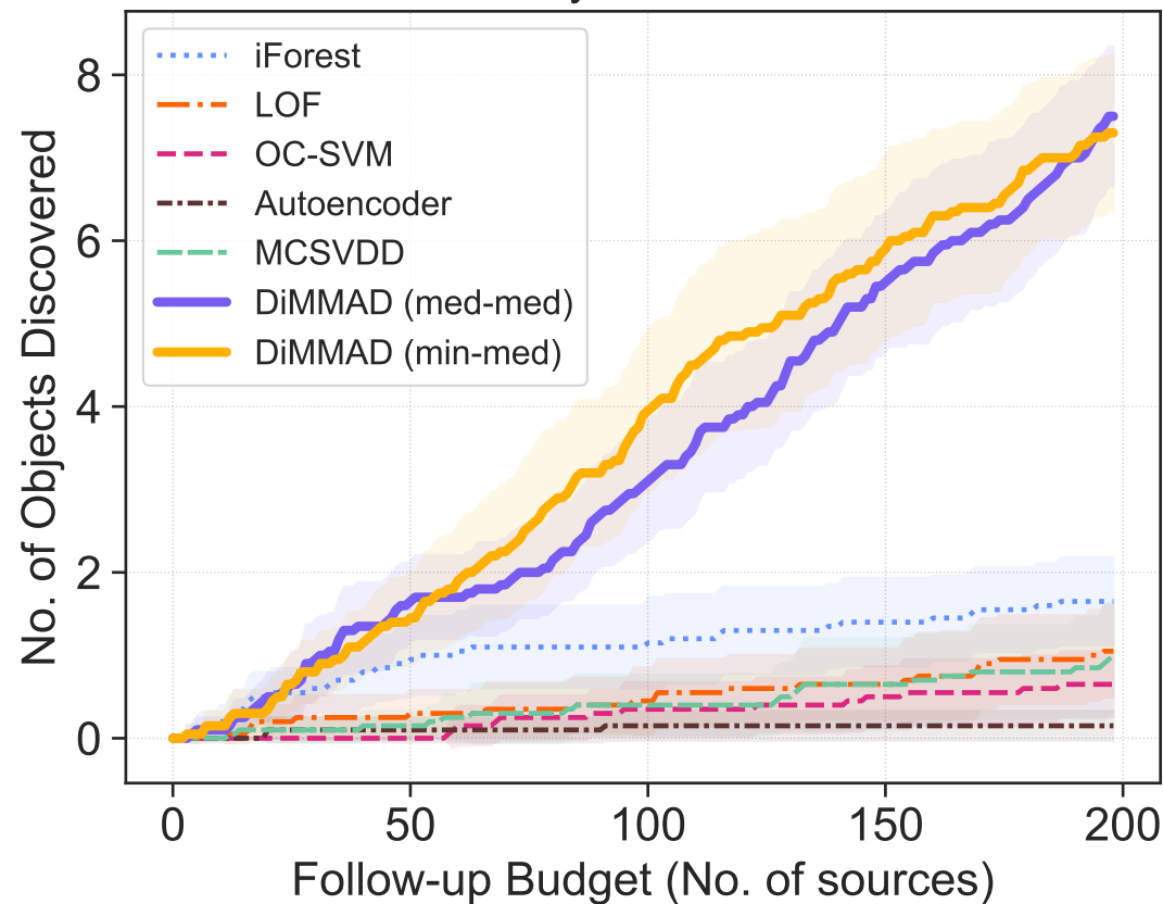
Anomaly: SNIa-SALT3
